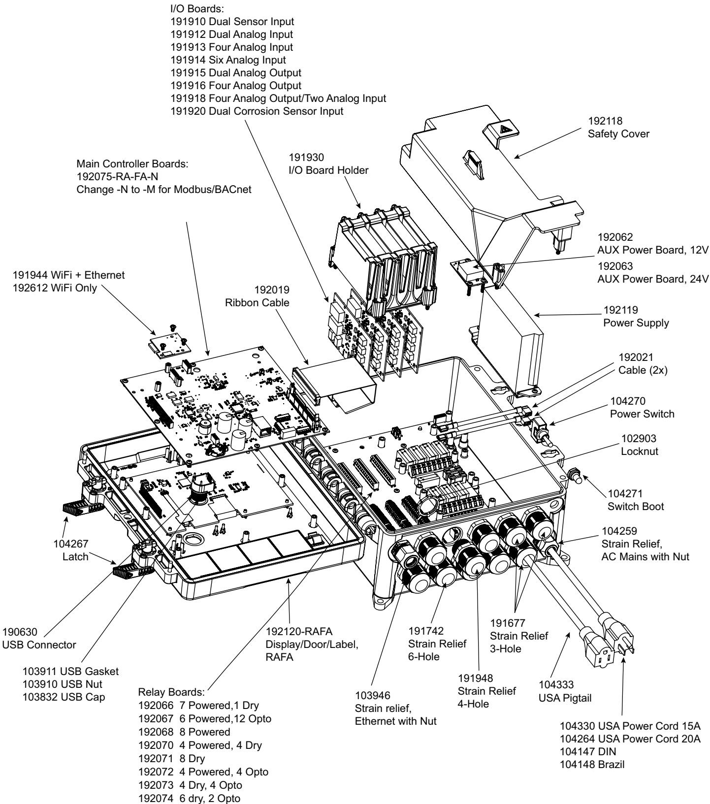
Controller Parts – Fixed Relays
